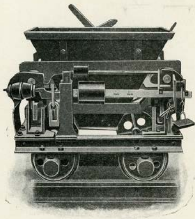
BASCULE-WAGONNET
