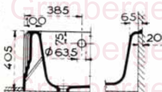
Section BB Section CC
